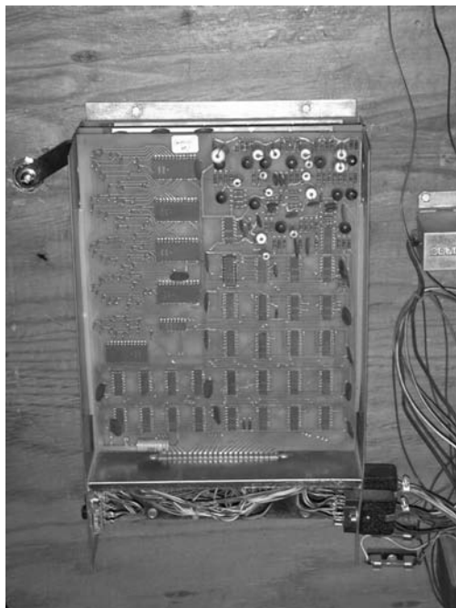
Figure 4. Circuit board, possibly from Computer Space, serial number 1. (Courtesy of http://www.computerspacefan.com/SN1large.htm )
