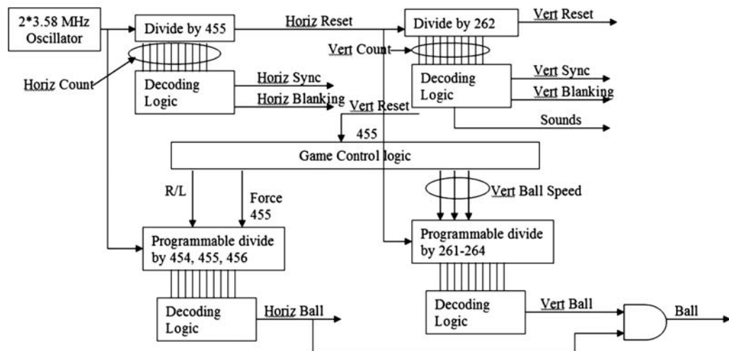
Figure 1. Al Alcorn's simplified block diagram for Pong. 4
